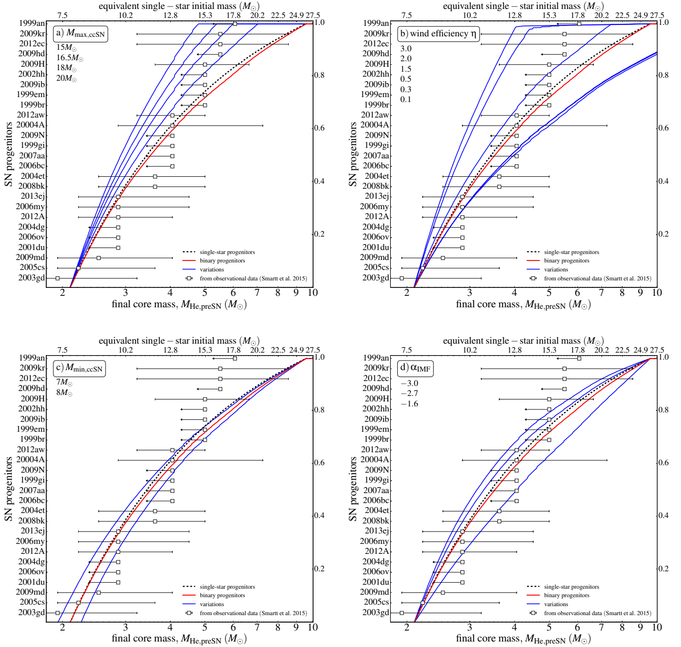
Fig. 6. Same as Figure 5 (with logarithmic x-axis here), but showing the results for other varying assumptions (blue lines): a) the mass threshold for failed SN collapsing onto black holes M_{\max, \text{ccSN}} (Models 52, 53, 54 and 29), b) the wind mass loss efficiency \eta (Models 25, 26 and 51), c) the minimum mass for SN, M_{\min, \text{ccSN}} (Models 30 and 31) and d) the slope of IMF \alpha_{\text{IMF}} (Models 32 to 34). These physical parameters influence the whole population, both single stars and in binary systems. The list of values depicted in the upper left corner shows a sequence of the varying distributions (blue lines) spanning from top left to bottom right of each panel.
