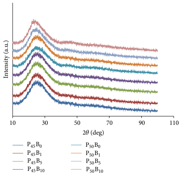
FIGURE 1: Powder X-ray diffraction pattern for glasses in the system of \text{P}_{45}\text{Ca}_{16}\text{Mg}_{24}\text{Na}_{(15-x)}\text{B}_x and \text{P}_{50}\text{Ca}_{16}\text{Mg}_{24}\text{Na}_{(10-x)}\text{B}_x .
