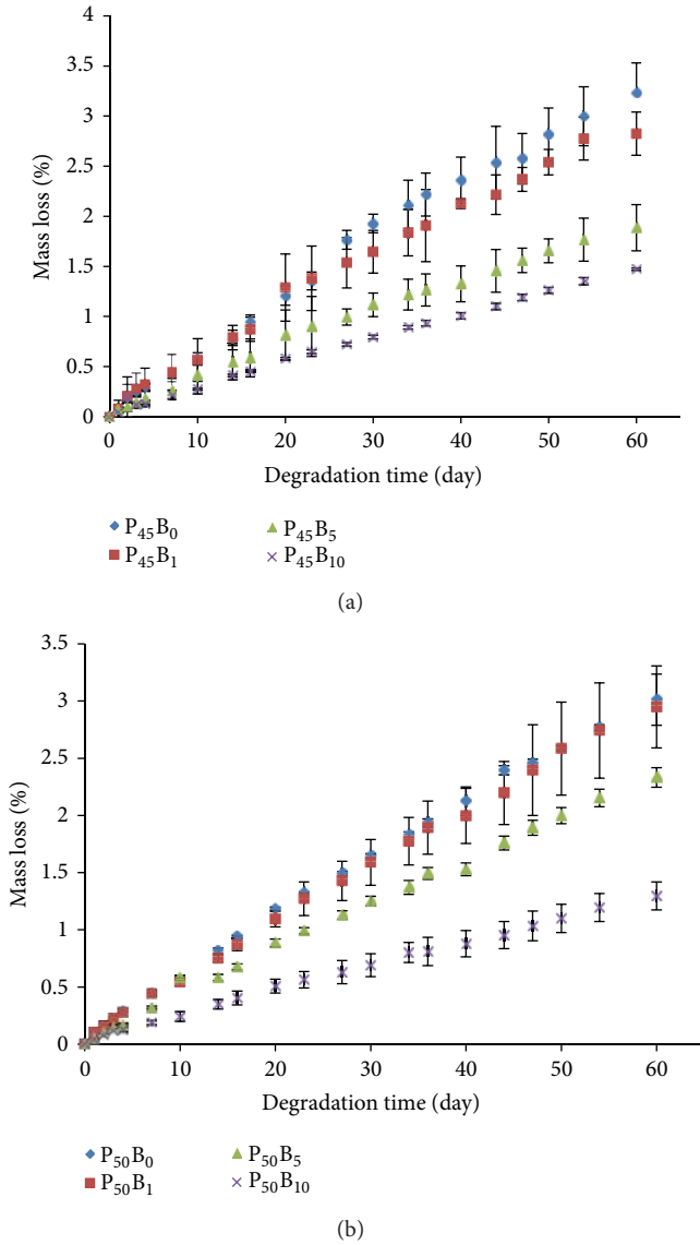
FIGURE 7: Plot of mass loss (%) of the glasses in the system of (a) P_{45}Ca_{16}Mg_{24}Na_{(15-x)}B_x and (b) P_{50}Ca_{16}Mg_{24}Na_{(10-x)}B_x ( x = 0-10 ) in PBS at 37^\circ C for 60 days.
