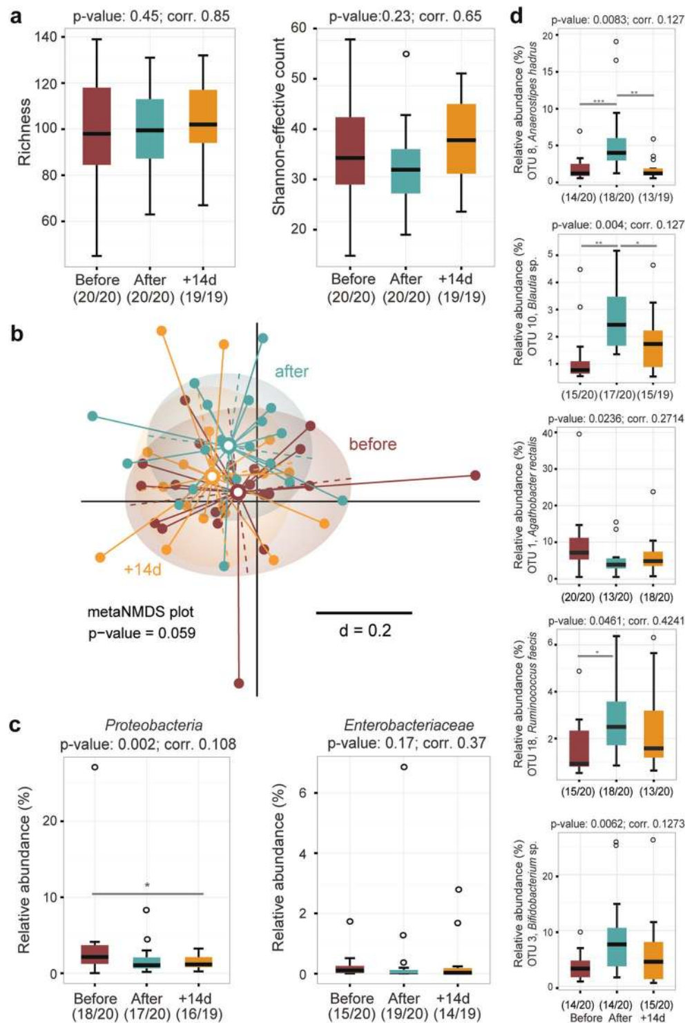
Figure 2. Fecal microbiota analysis by 16S rRNA gene amplicon analysis. (a) Diversity within samples ( alpha -diversity) was estimated by species richness and Shannon-effective counts. (b) meta nonparametric multidimensional scaling plot of phylogenetic distances based on generalized UniFrac ( beta -diversity). (c) Occurrence of members of the phylum Proteobacteria and the family Enterobacteriaceae , including significance before and after Benjamini-Hochberg adjustment. (d) Relative abundances of five dominant OTUs showing significance overtime. *** P < 0.001 ; ** P < 0.01 ; * P < 0.05 .
