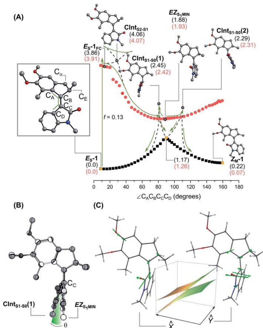
Fig. 6 Excited state isomerisation of E_S-1 . (A) Optimised S_0 and S_1 profiles along the rotation coordinate identified by the C_A C_B C_C C_D dihedral angle at the XMS-CASPT2/6-31G*///CASCF(12,12)/6-31G* level of theory. The relative energies in eV of the stationary points and Clnts found along the relaxed scan are reported in parentheses (black: gas phase; red: single point using the PCM model for methanol). (B) Superposition of the geometry of EZ_{S_1-MIN} (in white) and Clnt_{S_1-S_0}(1) (in grey). The two structures mainly differ for their degree of pyramidalisation ( \angle \theta ) of C_C of the lower half. (C) Depiction of the branching plane of Clnt_{S_1-S_2}(1) with the vectors \hat{x} and \hat{y} highlighted. Vector \hat{x} features the pyramidalisation distortion typical of the alkene branching plane, while vector \hat{y} describes the C_B=C_C bond twisting associated with the rotation. The sloped nature of the Clnt can be appreciated by the tilting in the \hat{x} direction.
