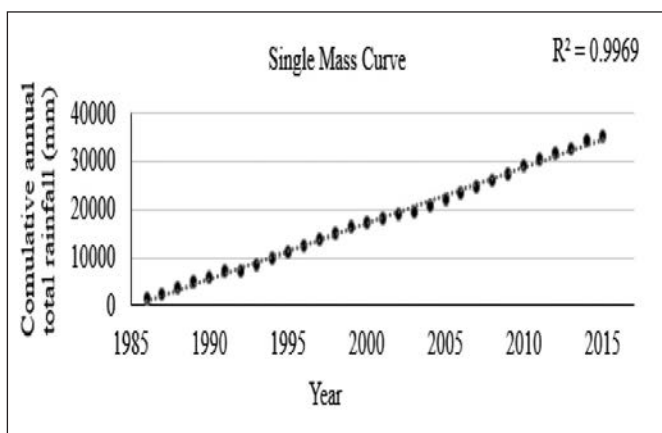
Fig. 2: Single mass curve on rainfall data for Indibir station
