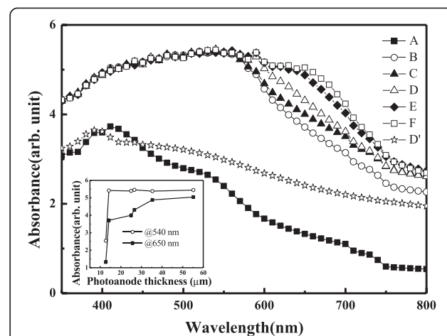
Figure 3 The UV-vis absorption spectra of compressed \text{TiO}_2 NP thin films with various thicknesses. Samples A to F have a photoanode thickness of 12.7, 14.2, 25.0, 26.6, 35.3, and 55.2 \mu\text{m} , respectively, with dye adsorption. Sample D' is the \text{TiO}_2 NP thin film of 26.6 \mu\text{m} in thickness (the same as sample D) but without dye adsorption.
