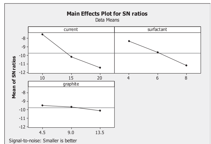
Fig. 5. S/N response graph for surface roughness.
