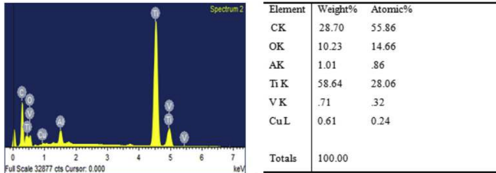
Fig. 10. EDS Analysis of with machined titanium alloy.
