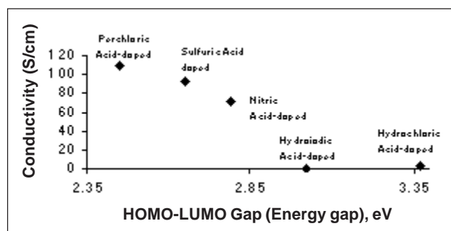
Fig. 4. Conductivity versus HOMO-LUMO gap plot of the PANi-ES samples with different dopants.
