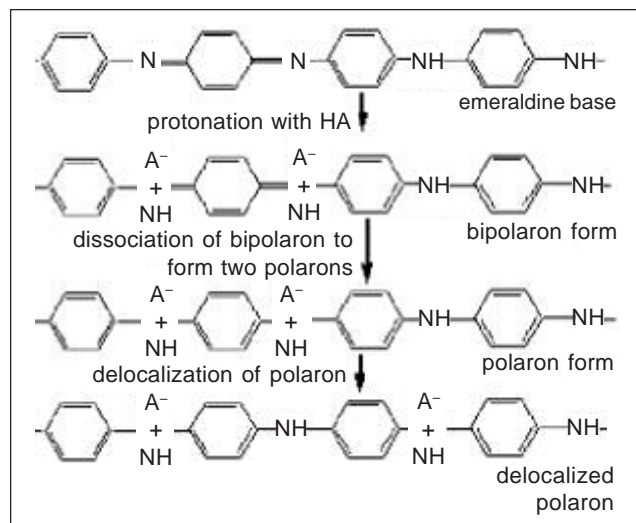
Fig. 1. Protonic acid doping of polyaniline (emeraldine base) (Trchova et al., 1998).
