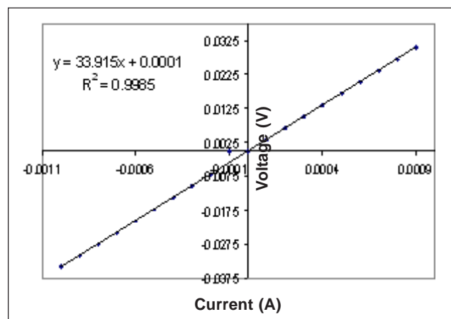
Fig. 2. I - V curve of PANi-ES with \text{HClO}_4 dopant showing symmetry from -1 to 1 mA.
