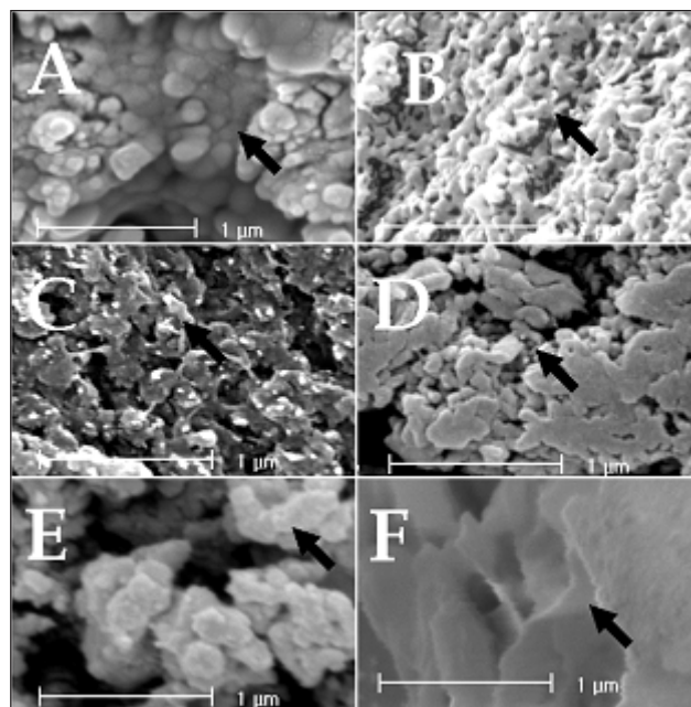
Fig. 5. SEM images at ~26000x magnification of (A) undoped PANi, (B) HCl-doped, (C) HNO 3 -doped, (D) HClO 4 -doped, (E) H 2 SO 4 -doped, and (F) HI-doped polyaniline samples showing distinct structures pointed by arrows.
