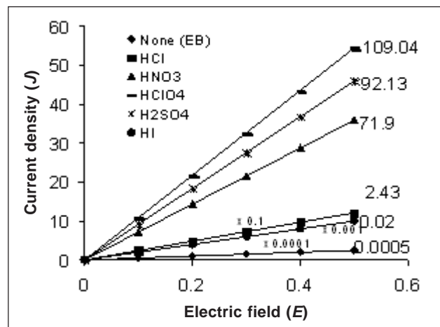
Fig. 3. Scaled plots of current density versus electric field for PANi-ES with different dopants showing the slopes as the conductivity in S/cm.
