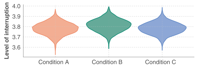
Fig. 11. Posterior distribution for self-reported level of interruption.
