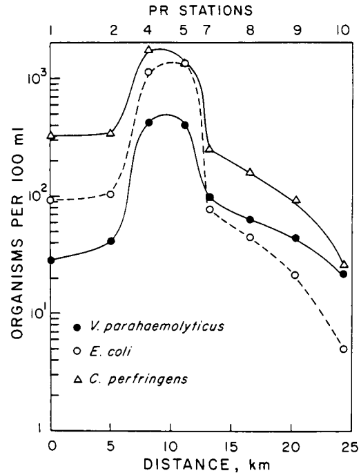
FIG. 3. Relationship of V. parahaemolyticus densities to those of E. coli and C. perfringens at selected Providence River stations.
