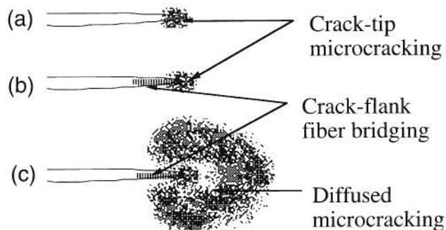
Fig. 1. Fracture process zone in (a) brittle cement, (b) quasi-brittle concrete and FRC, and (c) ductile ECC.
