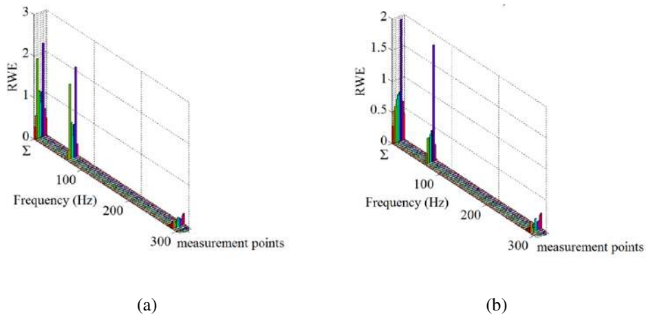
Figure 14: Scale-dependent RWE(j) in (16) and RWE in (10) (denoted by \Sigma ) using a 128-scale harmonic wavelet filter bank (3.91Hz bandwidth per scale) for the space truss of Figure 6 subject to (a) the sine-sweep and (b) the white noise excitation in Figure 8.
