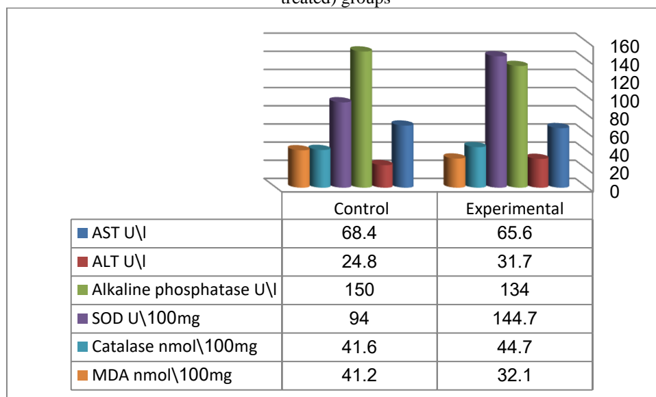
Fig.2: Mean Values of Liver Enzymes and MDA Concentration in the Control and Experimental (gum Arabic treated) groups
