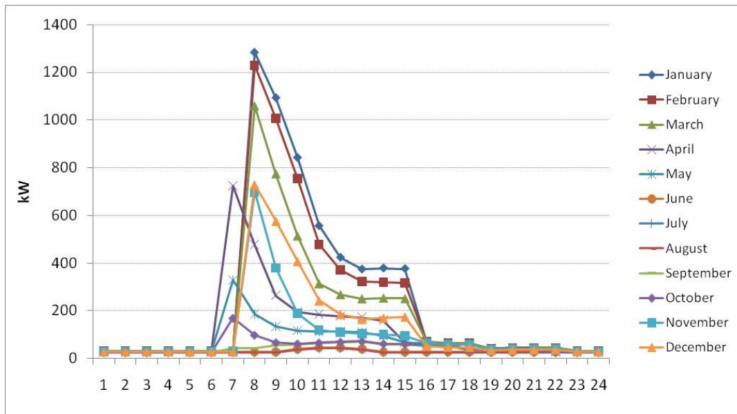
Figure 14. NYC school weekday total heat (space + water heating) demand 17
