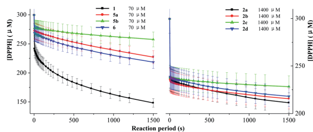
Fig. 5 Decay of 299.51 μM DPPH in the presence of DDMP derivatives.
