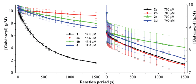
Fig. 6 Decay of 10.95 μM galvinoxyl in the presence of DDMP derivatives.
