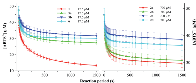
Fig. 4 Decay of 47.69 μM ABTS •+ in the presence of DDMP derivatives.
