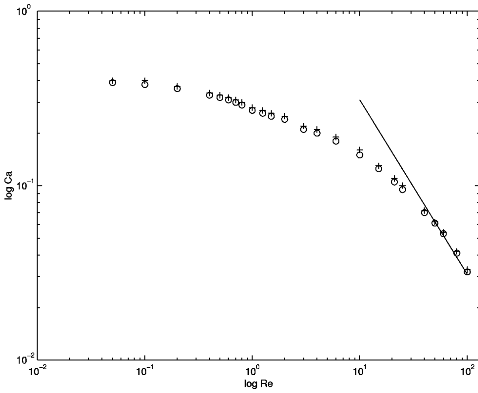
FIG. 1. Log-log plot of Re vs Ca, \lambda = 1 , equal densities. + drop breakup, O steady state solution, — line. Re.Ca = \text{constant} .
