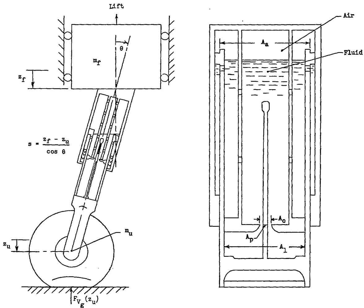
(a) System with two degrees of freedom.
