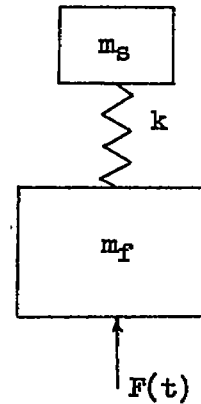
(b) Concentrated-mass system.
