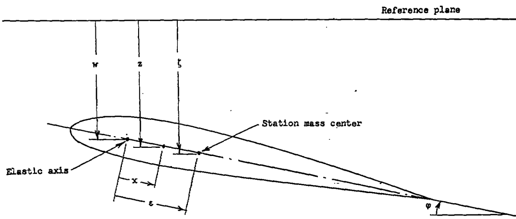
(b) Coordinates at any transverse station.
