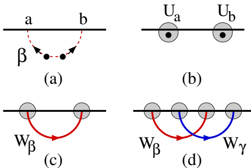
FIG. 1. (a) We consider a thought experiment in which we create two Z_2^\perp fluxes in the bulk and then move them along a path \beta to points a, b at the edge. (b) We argue that the two fluxes can be annihilated at the boundary by applying local operators U_a, U_b . (c) We define \mathbb{W}_\beta to be an operator which describes a process in which the fluxes are created in the bulk, brought to the edge, and then annihilated. (d) To obtain a contradiction, we consider two paths \beta, \gamma that intersect one another, and we investigate the commutation algebra of the corresponding operators \mathbb{W}_\beta, \mathbb{W}_\gamma .
