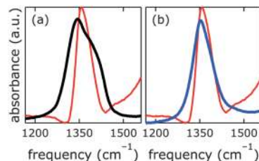
Fig. 7 Infrared spectra of [NiFe]-( \text{NO}_3^- )-LDH nanosheets as synthesized (black), after being suspended in carbonate-free strong base electrolyte in Ar atmosphere as described above (blue), and after being suspended in 0.1 M aqueous KOH in ambient air (red).
