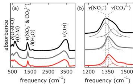
Fig. 6 Infrared spectra of [NiFe]-( \text{NO}_3^- )-LDH nanosheets as synthesized (black), after being suspended in 0.1 M aqueous \text{K}_2\text{CO}_3 solution (grey), and after being suspended in 0.1 M aqueous KOH (red); (a) full spectra, (b) magnification of the region characteristic for \text{NO}_3^- and \text{CO}_3^{2-} . Lorentzian fits are depicted as thin lines.
