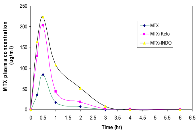
Fig. 1: The mean plasma MTX concentrations observed after injection of MTX (50 mg/kg, i.p) to eight different mice in the three treatment groups.
