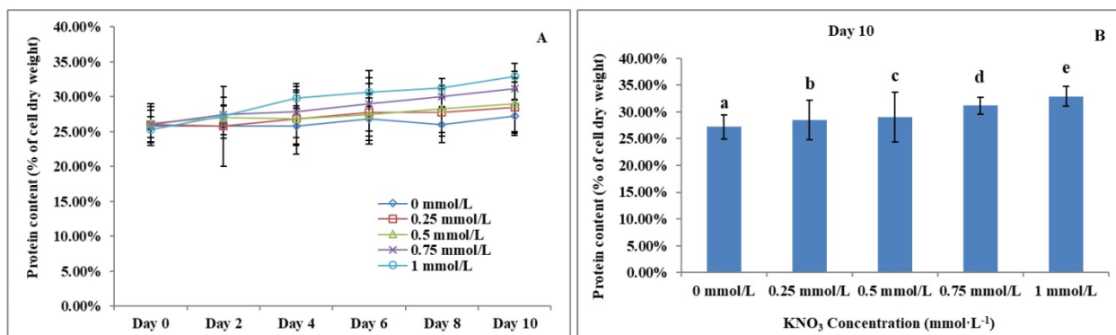
Figure 8. (A) Ten days' protein content trend of P. dentata growing in f/2 medium containing different concentrations of KNO 3 (0, 0.25, 0.5, 0.75, and 1 mmol L -1 ); (B) Protein content of P. dentata in different KNO 3 concentration culture mediums on day 10. [Note: a b c d e alphabets indicates the significant difference (P<0.05) among the test conditions, given by Duncan's multiple range test].
