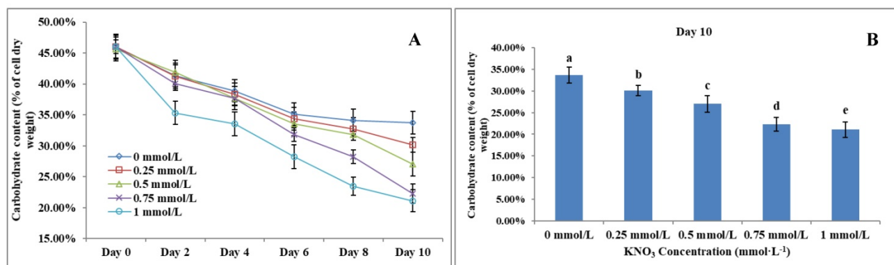
Figure 7. (A) Ten days' carbohydrate content trend of P. dentata growing in f/2 medium containing different concentrations of KNO 3 (0, 0.25, 0.5, 0.75, and 1 mmol L -1 ); (B) Carbohydrate content of P. dentata in different KNO 3 concentration culture mediums on day 10. [Note: a b c d e alphabets indicates the significant difference (P<0.05) among the test conditions, given by Duncan's multiple range test].
