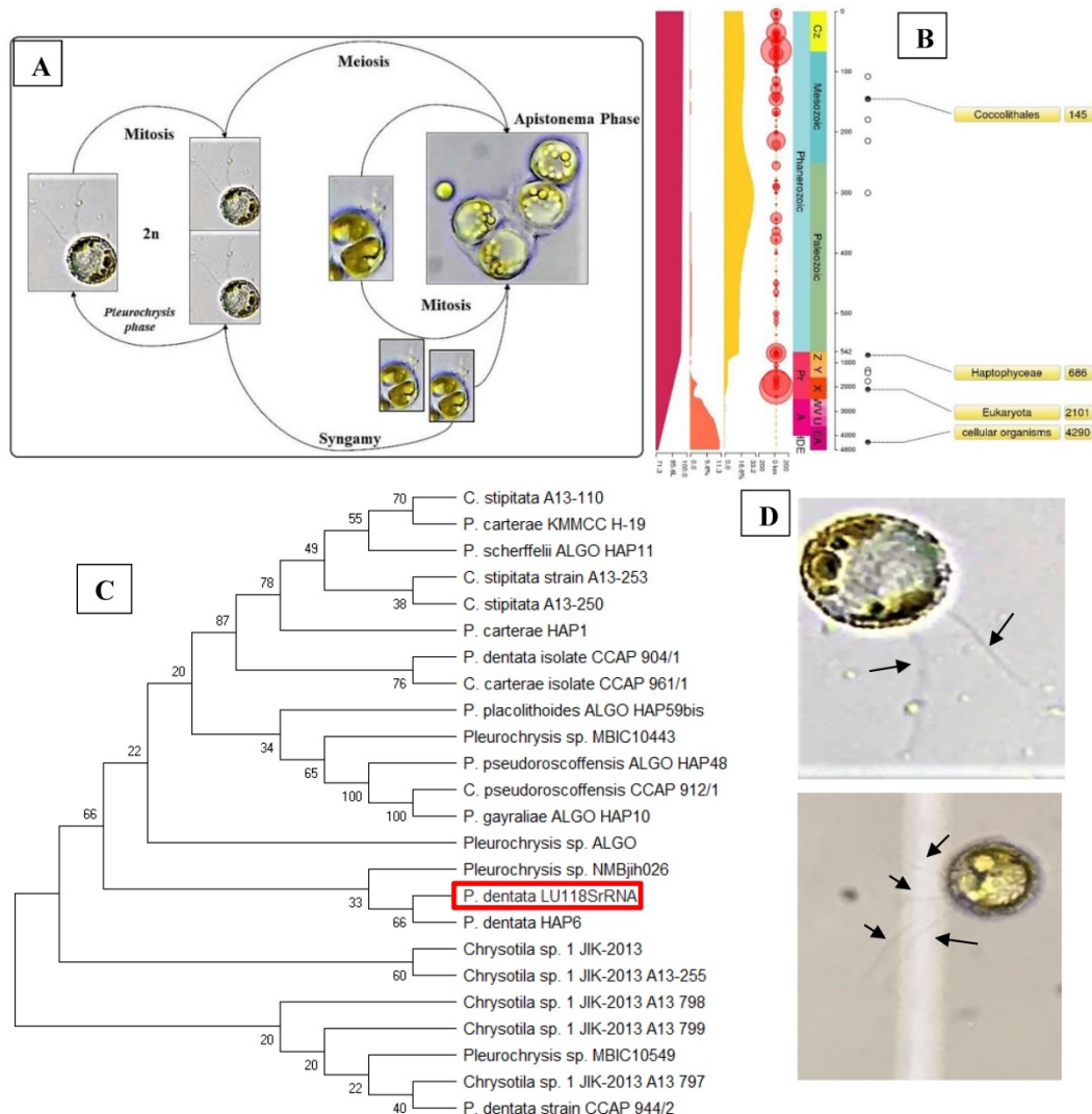
Figure 1. (A) Compound microscopy images of P. dentata life cycle showing alternation of generations; (B) TimeTree analysis of Pleurochrysis genus; (C) phylogenetic analysis of Pleurochrysis sp. 18S rRNA; (D) compound microscopic images showing fully developed P. dentata with two and four flagella.
