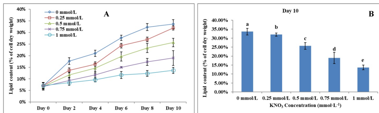
Figure 6. (A) Ten days' lipid content trend of P. dentata growing in f/2 medium containing different concentrations of KNO 3 (0, 0.25, 0.5, 0.75, and 1 mmol L -1 ); (B) Lipid content of P. dentata in different KNO 3 concentration culture mediums on day 10. [Note: a b c d e alphabets indicates the significant difference (P<0.05) among the test conditions, given by Duncan's multiple range test].
