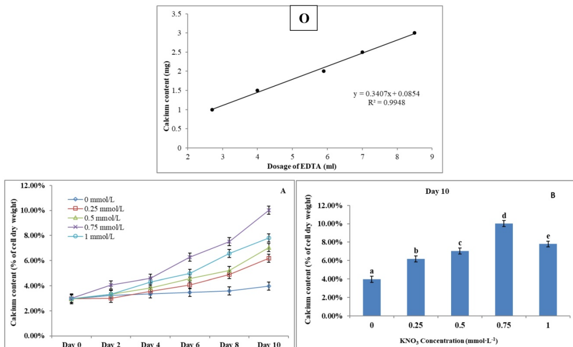
Figure 4. (O) Calcium ion content standard curve. (A) Ten days' calcium content trend of P. dentata growing in f/2 medium containing different concentrations of \text{KNO}_3 (0, 0.25, 0.5, 0.75, and 1 mmol L -1 ); (B) Calcium content of P. dentata in different \text{KNO}_3 concentration culture mediums on day 10. [Note: a b c d e alphabets indicates the significant difference ( P < 0.05 ) among the test conditions, given by Duncan's multiple range test].
