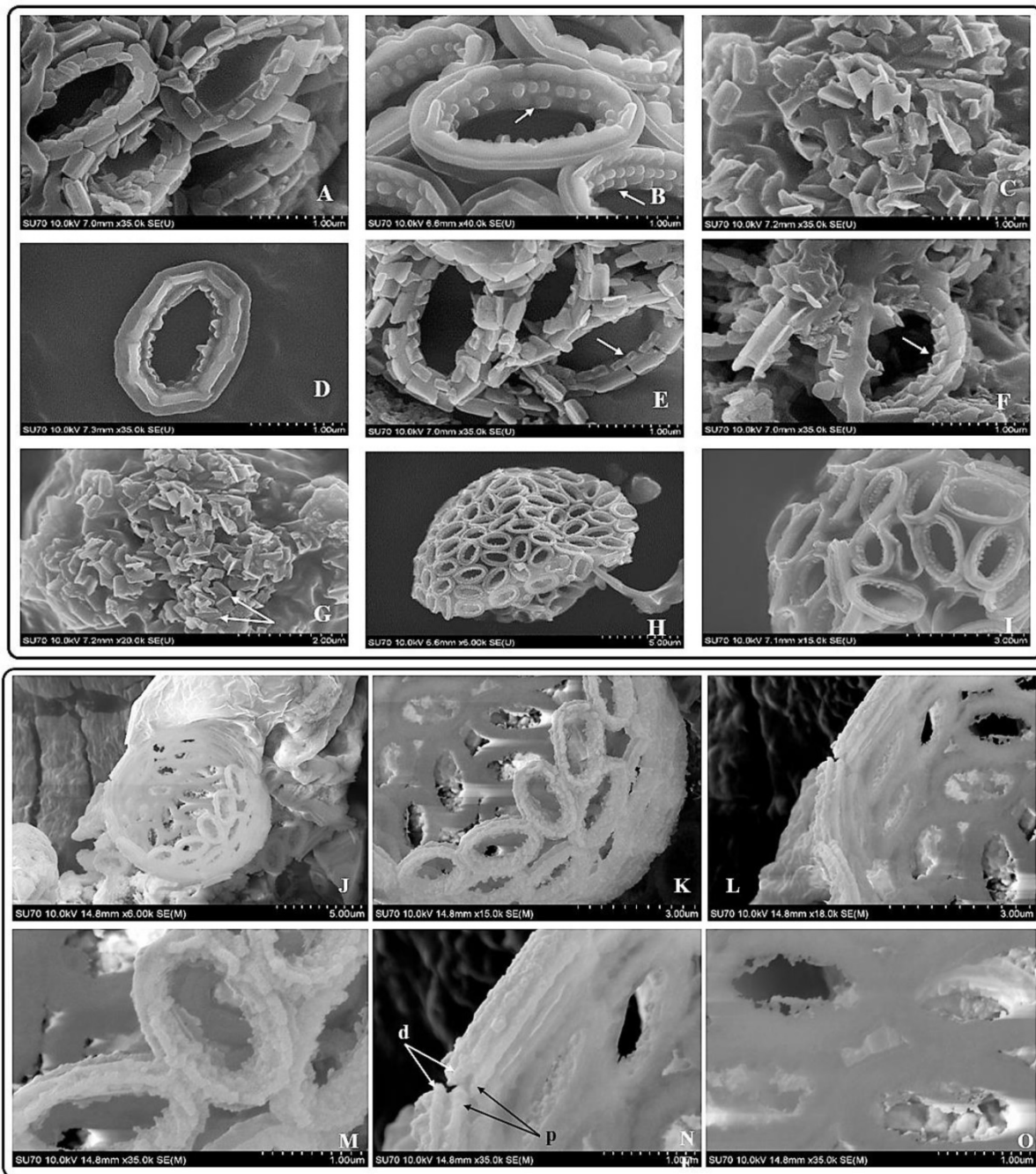
Figure 2. SEM pictures of P. dentata coccolith. (i) (A) Loose structure of coccolith. (B, E, F) The arrow points to "doornail structure". (C) Cracked coccolith. (D) Single coccolith. (G) The arrow points to "R unit". (H, I) P. dentata wrapped by coccolith. (ii) Support Structure of CaCO 3 cell wall. (J) an empty shell without protoplasts. (K) Close range view. (L) Adjacent two coccolith side views. (M) Top view of two adjacent coccoliths. (N) Enlarged side view of two adjacent coccoliths. (O) Rear view of several adjacent coccoliths. Arrowhead d: distal-shield. Arrowhead p: proximal-shield.
