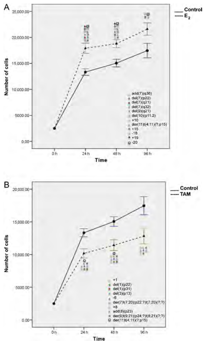
Figure 4 Effects of E_2 (A) and TAM (B) treatment for 24, 48, and 96 h on proliferation and corresponding chromosomal alterations in MCF7 cells. Error bars represent mean standard deviation of 24 separate experiments. Chromosomal abnormalities induced at each treatment time point are indicated. A full colour version of this figure is available at http://dx.doi.org/10.1530/ERC-16-0078 .
