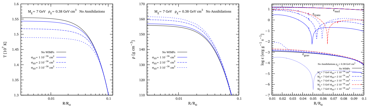
Figure 2: Impact of asymmetric DM on the Sun. Left Panel: Temperature profile of the Sun for different SD scattering cross-sections at t_\odot = 4.57 \text{ Gyrs} . Central Panel: Density profile (baryons only) inside the Sun. Right Panel: Energy transport (meaning of the curves as in Fig.1). The sign of \epsilon_{grav} is positive.
