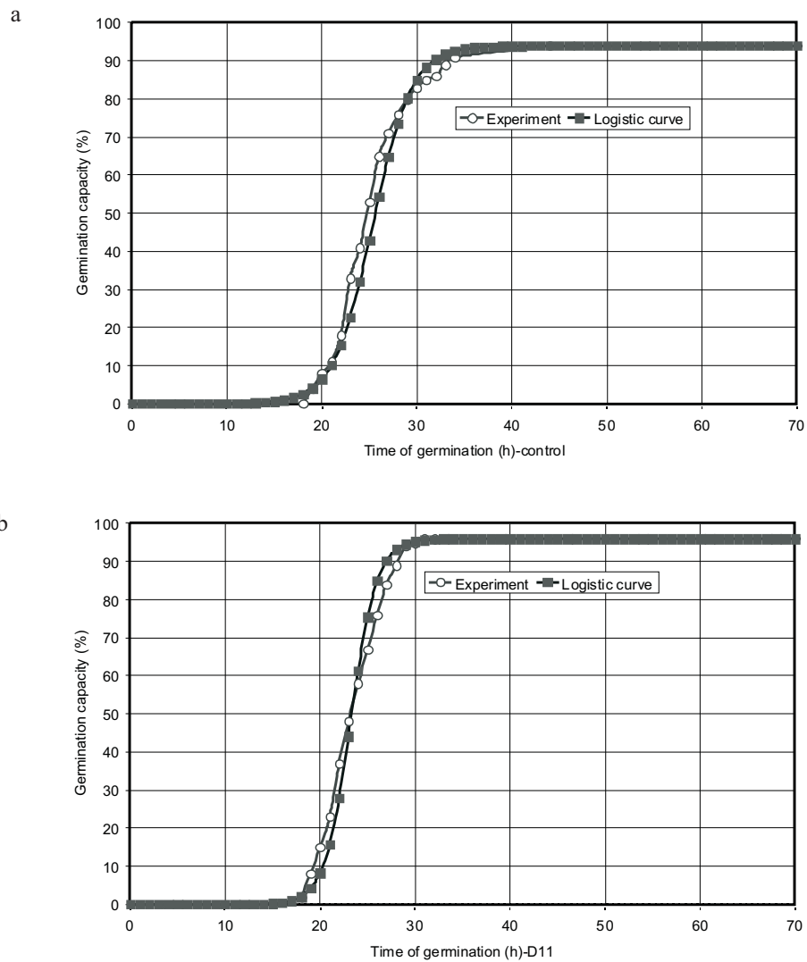
Fig. 2. Experimental data and the logistic curve for: a – control treatment; and doses: b – D11, c – D13, d – D21, e – D23.
