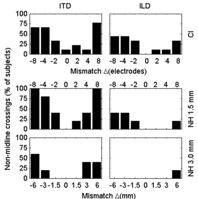
FIG. 5. A count of non-mid-line crossings for ITD and ILD lateralization is shown as a function of \Delta for CI and NH listeners. The numbers above the panels on the second row show the amount mismatch in terms of number of electrode spacing for the NH data.
