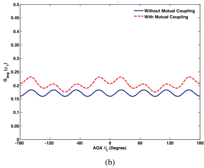
Figure 4. Variations of G_{avg}(\theta_1) for the “8 elements CA” with different radii, with and without MC; (a) r = 0.5\lambda ; (b) r = 0.7\lambda .
