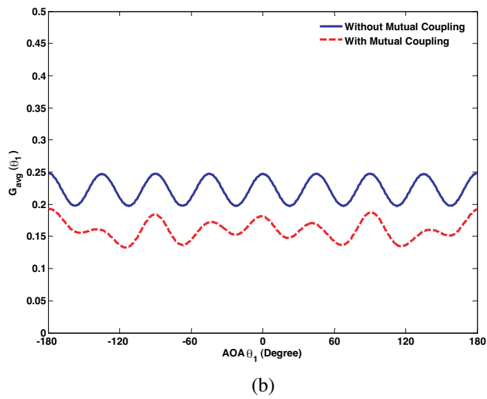
Figure 6. Variations of G_{avg}(\theta_1) for the “1 + 8 elements CA” with different radii, with and without MC; (a) r = 0.6\lambda ; (b) r = 0.8\lambda .
