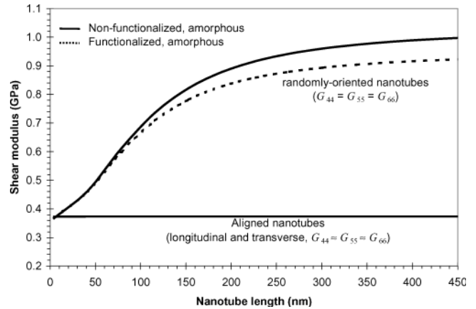
Fig. 6 Shear moduli G_{ij} of the composite systems vs nanotube length for a 1% nanotube volume fraction.
