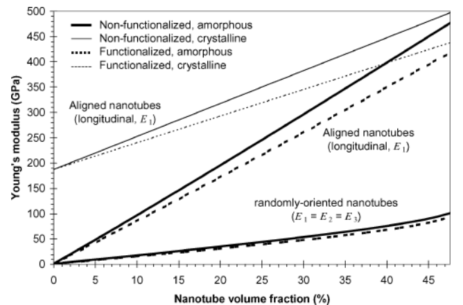
Fig. 7 Longitudinal Young's moduli E_1 of the composite systems vs nanotube volume fraction for a nanotube length of 400 nm.
