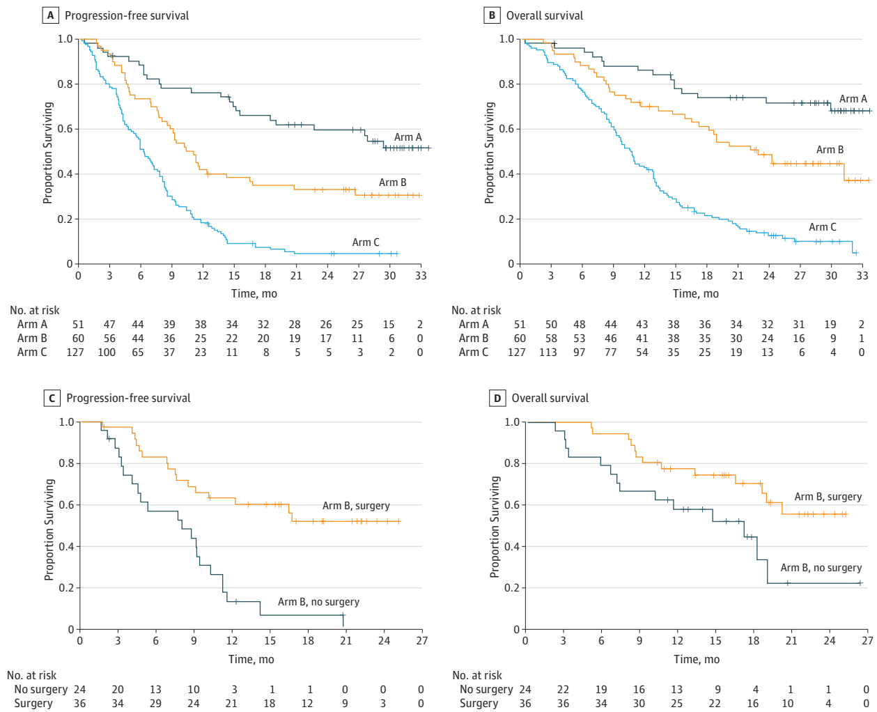
Figure 2. Survival Analyses
