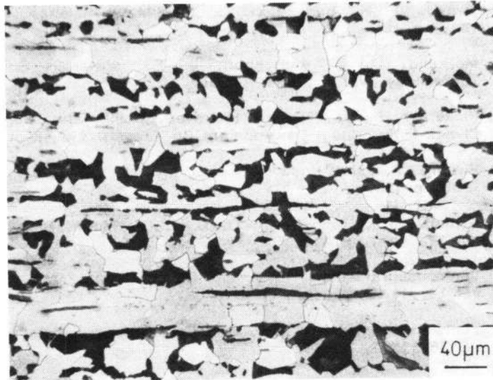
Figure 2 Banded pearlite in as-received steel
