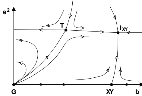
Fig. 1 – Schematic flow diagram of the quartic coupling b and the charge e^2 (see eq. (1)) at the critical surface T = T^* . Note the Gaussian ( G ), XY , inverted- XY ( I_{XY} ), and the tricritical ( T ) fixed points. Good type-I materials ( \kappa \ll 1 ) lie far to the left of the separatrix that connects the Gaussian and the tricritical fixed points.
