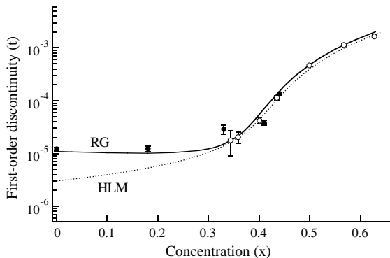
Fig. 2 – Size of the first-order NA transition ( t ) as a function of 10CB concentration ( x ) in the 8CB-10CB system. Comparison between the RG result (full line), HLM (dashed line), and experiment. Filled circles are data from Yethiraj and Bechhoefer, while hollow circles are latent-heat data from Marynissen et al. , converted into equivalent size t .
