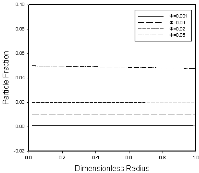
Fig. 3. Influence of the mean particle concentration on the concentration distribution. (Pe=2, Re_p=0.01 , a=2.5 , K_c=0.4 , K_\mu=0.6 ).
