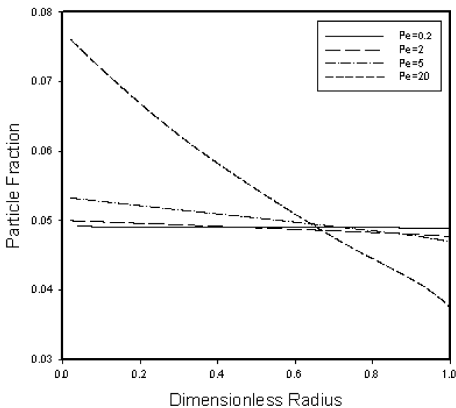
Fig. 2. Influence of the Peclet number on the concentration distribution.
