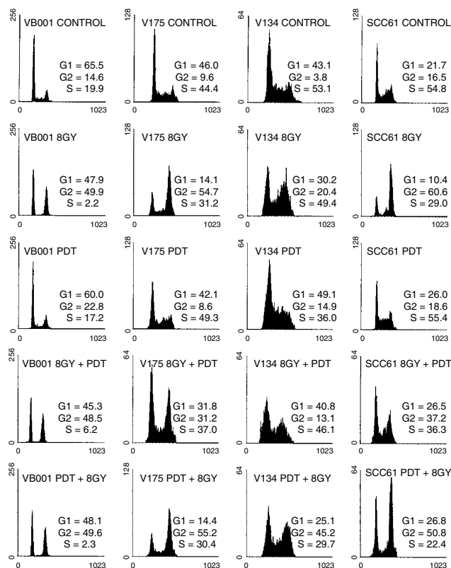
Figure 4 DNA histograms of the four cell lines used in this study. Cells were exposed to 8 Gy of ionizing radiation or 3 min of PDT or a combination of both treatments. Data represent distributions obtained from 5000 cells
