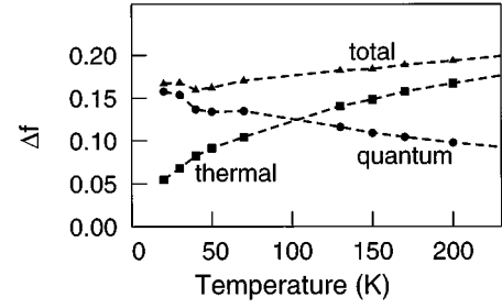
FIG. 2. Classical (squares), quantum (circles), and total (triangles) RMS fluctuation of the FE local-mode vectors [Eqs. (3) and (4)] in SrTiO 3 as a function of temperature.
