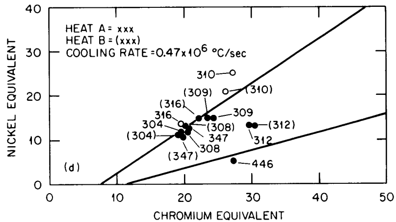
Fig. 15. Cooling rate modified Schaeffler diagrams showing the convergence of the 0 and 100% ferrite lines for the following cooling rates ( ^{\circ}\text{C}/\text{s} \times 10^{-6} ) (a) 0.07, (b) 0.12, (c) 0.28, (d) 0.47, (e) 0.71, (f) 1.1, (g) 1.2, (h) 1.4, (i) 1.8, (j) 2.3. Open symbols represent single phase structures and filled symbols represent duplex structures.
