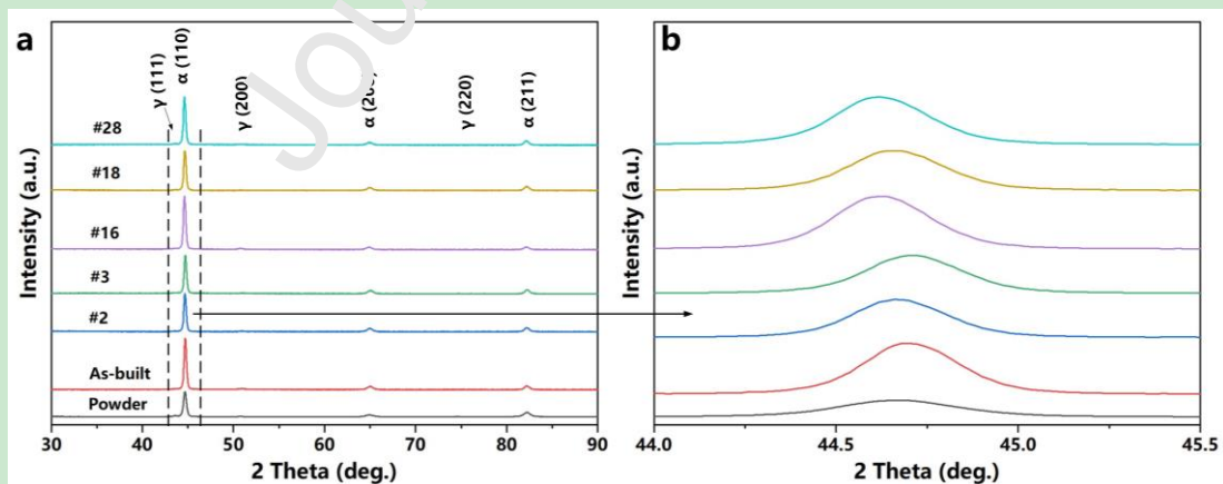
Fig. 8. XRD patterns of the 18Ni-300 maraging steel powder feedstock and the samples fabricated under the as-built and different remelting conditions.
