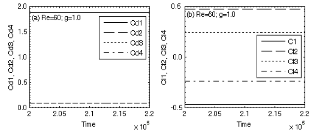
Fig. 8. Time signal analysis of drag and lift coefficients.
