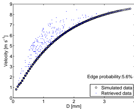
(b) Laser Precipitation Monitor
