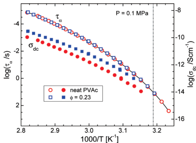
Figure 12. Local segmental relaxations times (open symbols) defined from the inverse of the peak frequency) for unfilled and filled PVAc; the \tau_\alpha(T) are seen to be equivalent. The solid line is the fit of eq 5 to the combined data. Also shown is the dc conductivity (filled symbols), which is larger in the PVAc containing silica due to a higher concentration of mobile ions. (Note the ordinate scale for \tau_\alpha is reversed to facilitate comparison with \sigma_{dc} .) The vertical dashed line designates the calorimetric T_g .
