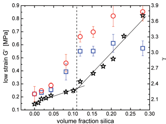
Figure 5. Variation with silica concentration of the storage modulus at strain amplitudes < 0.1\% (stars; left ordinate scale) and of the scaling exponent (right ordinate scale; squares calculated using the specific volume of the compound and circles using V corrected for the PVAc content). The vertical dashed line denotes the minimum filler concentration for formation on a silica network.
