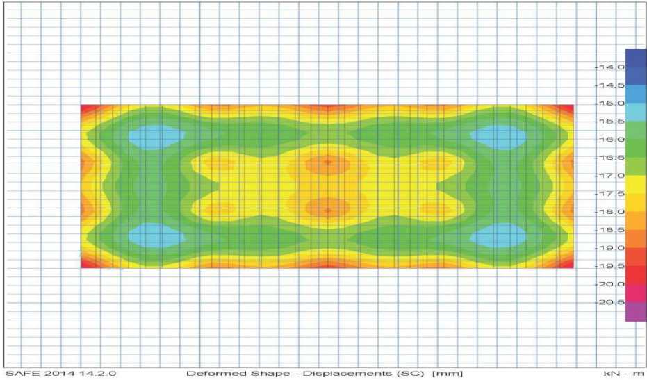
Fig. 6. Raft deformations ( K_s=10000 kN/m 3 ).
