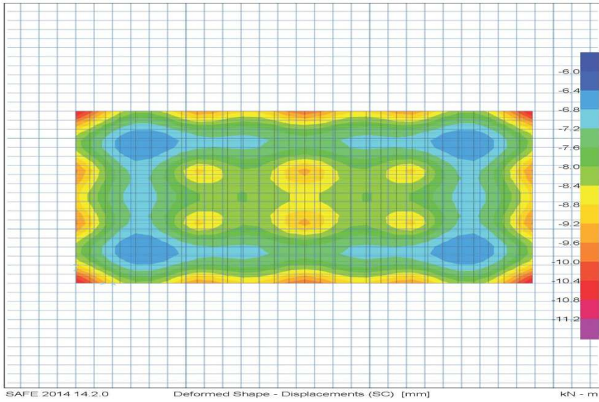
Fig. 8. Raft deformations ( K_s=21500 \text{ kN/m}^3 ).
