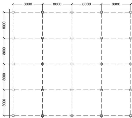
Fig. 2. Plan view of raft foundation for 10 story building
