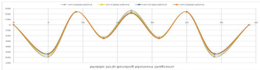
Fig. 4. Middle strip bending moment diagram
