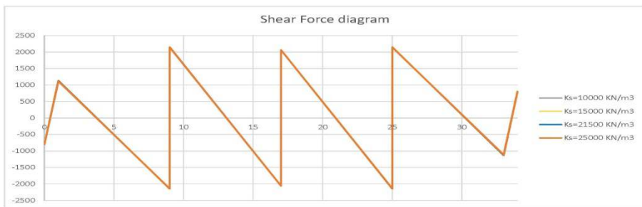
Fig. 5. Column strip Shear force diagram
