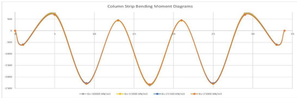
Fig. 3. Column strip bending moment diagram
