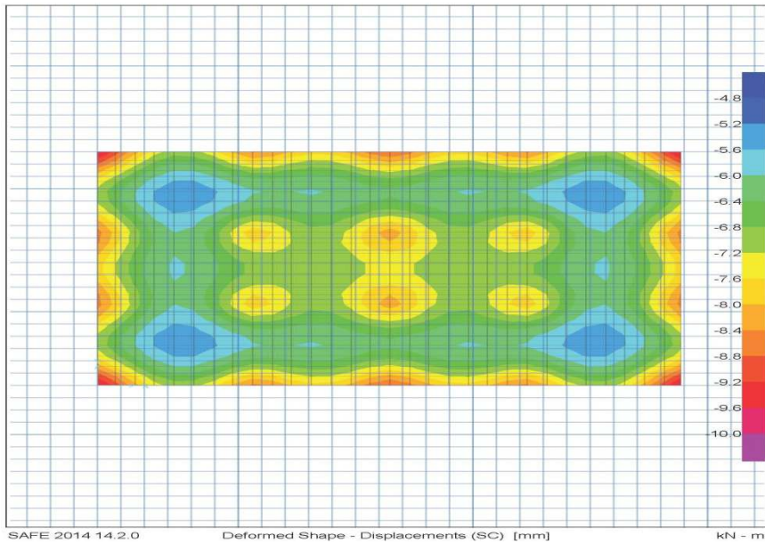
Fig. 9. Raft deformations ( K_s=25000 \text{ kN/m}^3 ).
