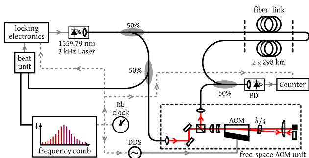
Fig. 4. Experimental setup for the characterization of the passive frequency stability of the fiber link (Amsterdam). For the long round-trip measurements, the free-space AOM unit (300 MHz) was replaced by a fiber-coupled AOM ( -42 MHz). In both cases the AOM was driven by a Rb-referenced DDS unit with a set accuracy of \sim 3.55 \mu\text{Hz} . Frequency deviations of the link are recorded with a Rb-referenced counter.
