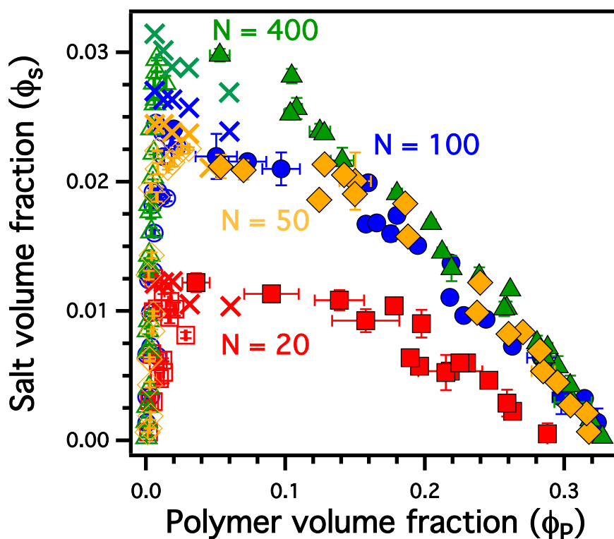
Figure S1. Experimentally determined phase diagrams of PLK-PRE system. The solid (complex phase) and open (supernatant phase) red squares, yellow diamonds, blue circles, and green triangles were the results obtained from TGA measurements for PLK-PRE systems with chain length of 20, 50, 100, and 400 repeat units, respectively. The red, yellow, blue, and green crosses were the results converted from calculation based on salt resistance concentration measurements. Reprinted (adapted) with permission from L. Li et al. , Macromolecules 51,8 (2018). Copyright (2018) American Chemical Society.
