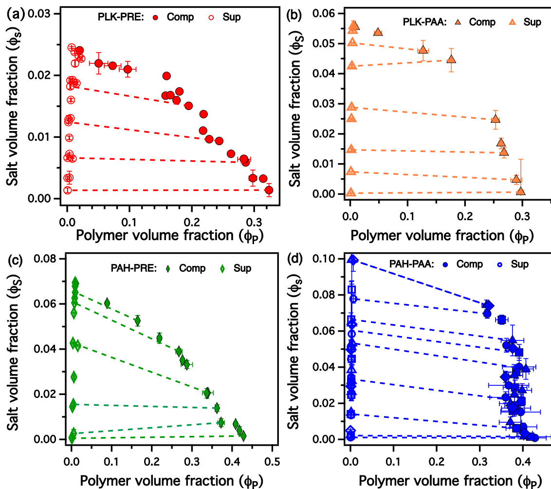
Figure S2. Individual phase diagrams of PLK-PRE (red), PLK-PAA (orange), PAH-PRE (green), and PAH-PAA (blue) systems. Selective tie-lines were drawn connecting complex phases (solid symbols) and corresponding supernatant phases (open symbols).
