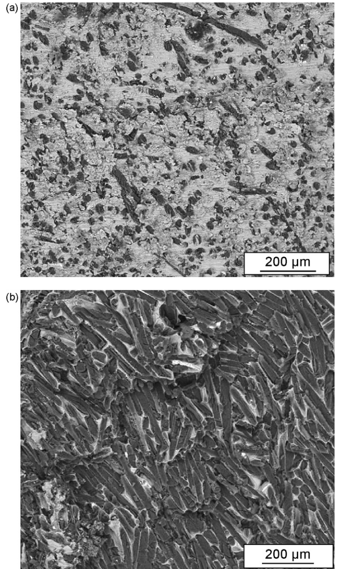
Fig. 13. SEM micrographs of the fractured ring part of a C_{PAN}/Al-Mg specimen (fibers perpendicular to loading direction): (a) low magnification of the external surface of undeformed specimen showing fibers distributed uniformly and (b) fracture surface in the region where the volume fraction of fibers (dark rods) is much higher than 30%.
