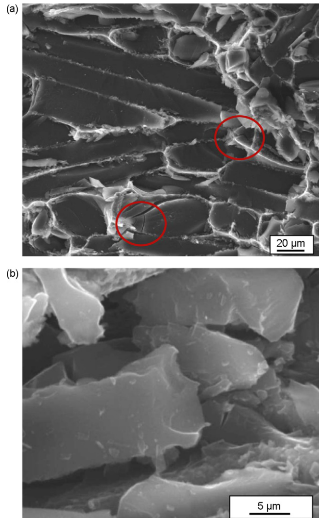
Fig. 11. Micrographs of fractured PAN-based carbon fibers in C_{PAN}/Al-Mg specimens (fibers parallel to loading direction) show (a) cracks of fibers and (b) rough and granular texture of fibers.
