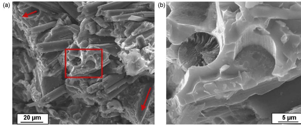
Fig. 9. Microstructure of a hat-shaped C_{Pitch}/Al-Mg specimen (fibers parallel to loading direction): (a) low magnification fracture and pull-out (indicated by arrows) of fibers and (b) high magnification shows fractured fibers.
