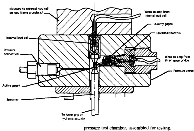
Fig. 2—Sectional view of pressure test chamber, assembled for testing.
