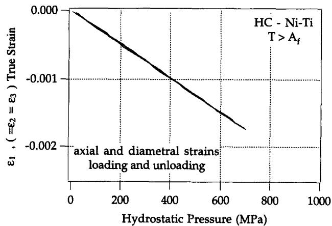
Fig. 4—HC stress state, true axial, and diametral strain vs hydrostatic pressure.
