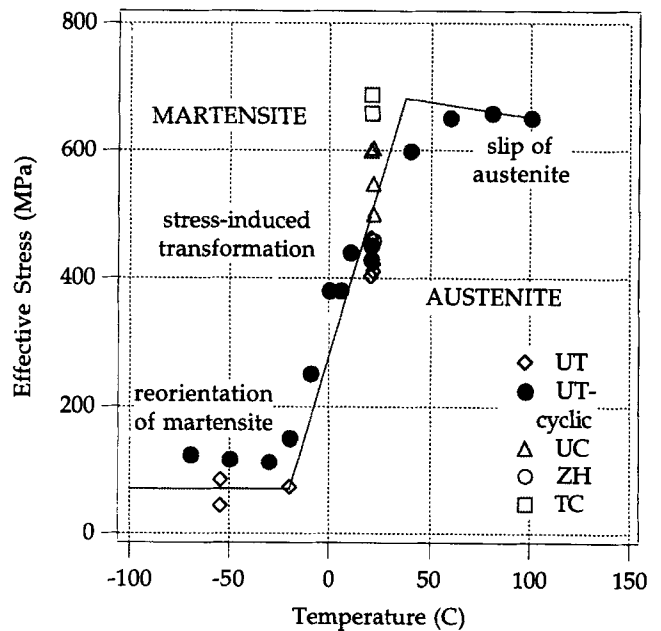
Fig. 9—Variation of effective stress for transformation vs temperature showing the increase in stress required for transformation with increasing temperature.
