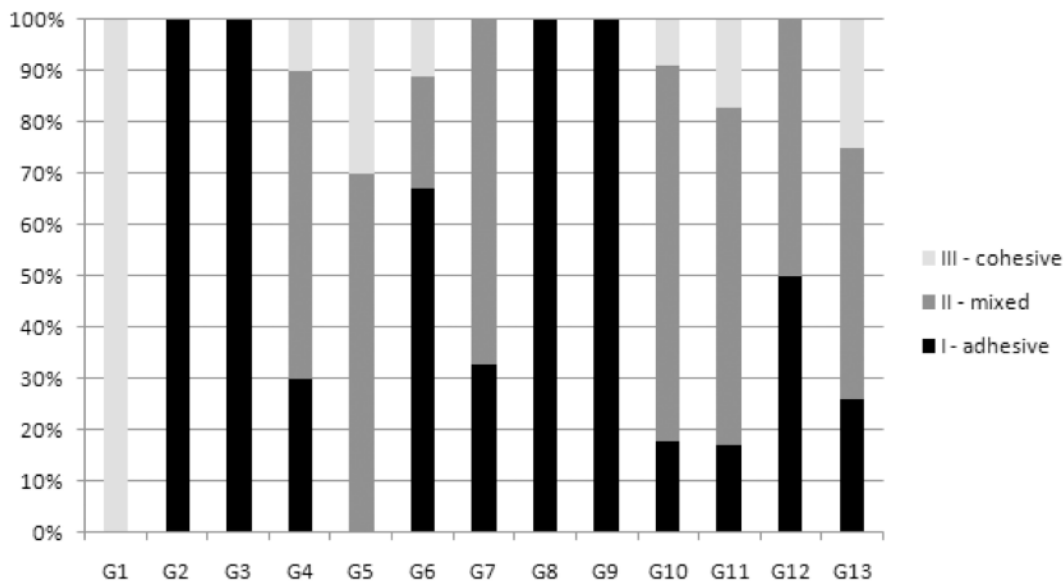
Fig. 2 Distribution of failure types per group. Type I: Adhesive failure at the interface; Type 2: Mixed failure (a combination of more than one type of fracture); Type III: Cohesive failure in the substrate composite. See Table 2 for group descriptions.
