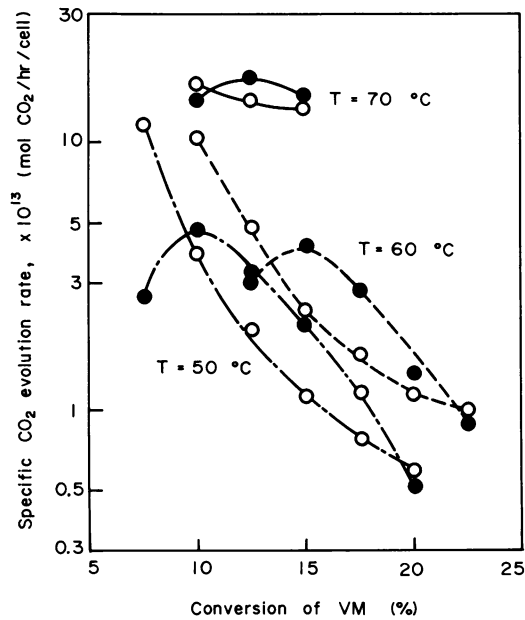
FIG. 6. The estimated specific CO 2 evolution rate at three different temperatures. Symbols: ○, thermophilic bacteria; ●, thermophilic actinomycetes; ---, 50°C; - - - -, 60°C; —, 70°C.
