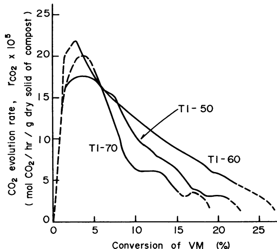
FIG. 4. CO 2 evolution rate versus conversion of VM at three different temperatures. The broken lines show the region where this temperature was below the setting temperature.
