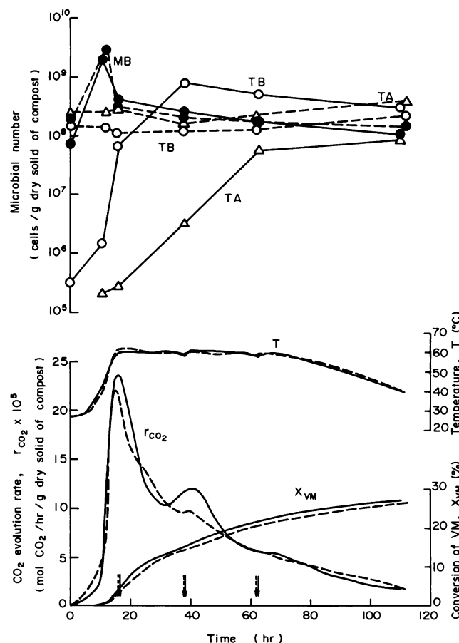
FIG. 2. Time courses of composting at 60°C (Runs T1-60 and T2-60). For the key to cell numbers and remarks, see the legend to Fig. 1.
