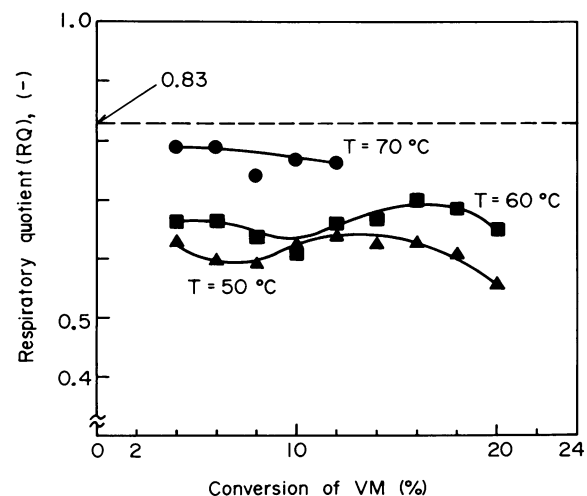
FIG. 8. RQ for each conversion of VM at three different temperatures. Symbols: ▲, 50°C; ■, 60°C; ●, 70°C.
