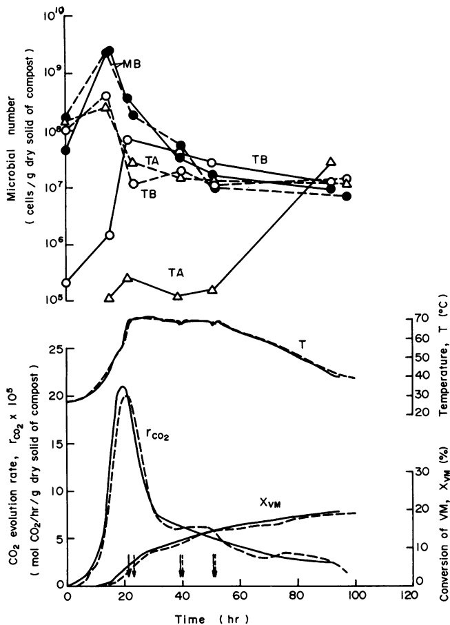
FIG. 3. Time courses of composting at 70°C (Runs T1-70 and T2-70). For the key to cell numbers and remarks, see the legend to Fig. 1.
