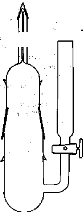
FIGURE 1. Dilatometer.
