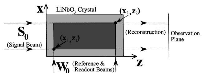
Fig. 1. 90^\circ geometry.
