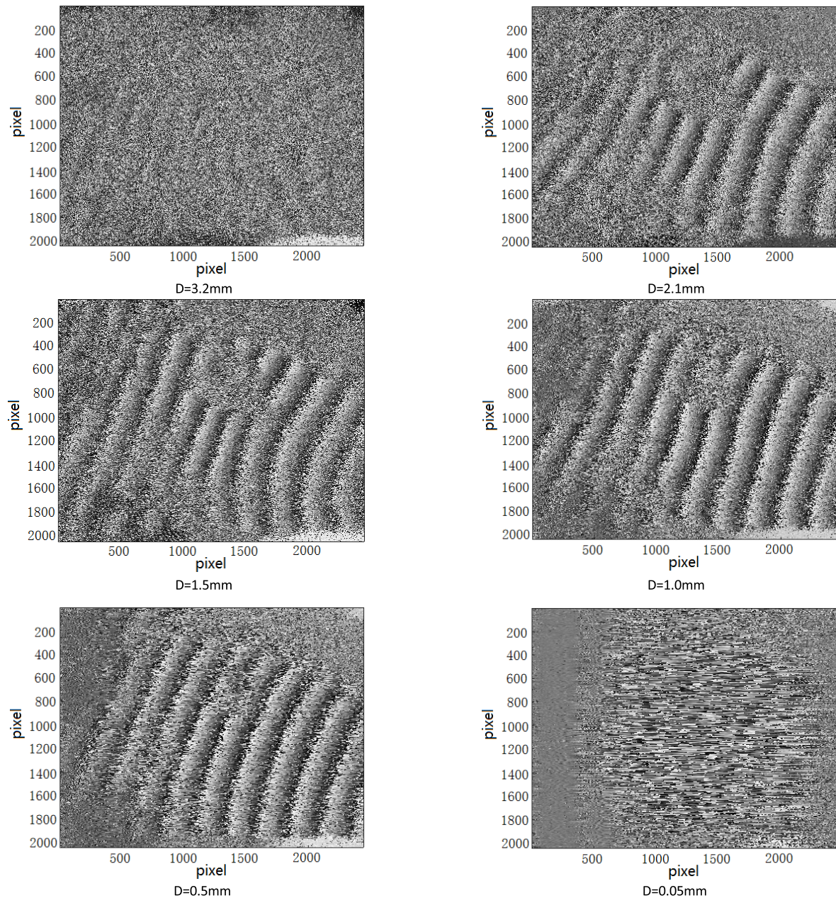
FIGURE 12. The phase maps of sample 2 corresponding to 5\mu\text{m} displacement loading under different aperture slit size.
