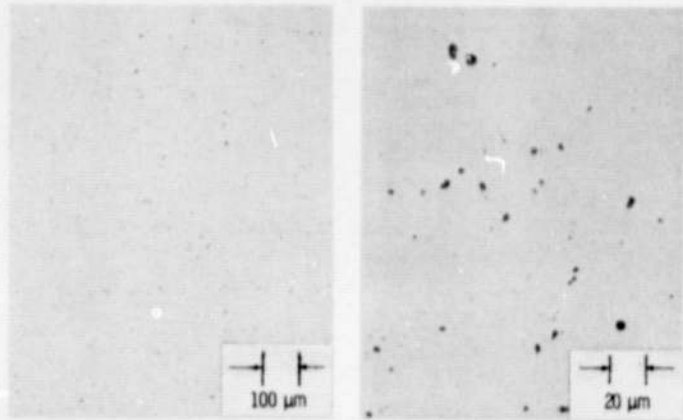
Figure 3. - Microstructure of porous pressing rim. UNETCHED
