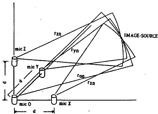
FIG.1. An image-source location. The location of an image source is the intersection of sphere surfaces. The radii are r_{0i} , r_{xi} , r_{yi} , and r_{zi} , respectively.
