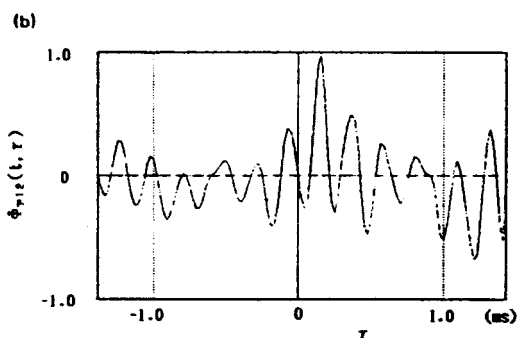
FIG.5. (a) Image-sources distribution, rise of sound field ( t : 0-3ms). (b) Cross-correlation function [see Eqs. (8) and (9)], rise of sound field ( t : 0-3ms).
