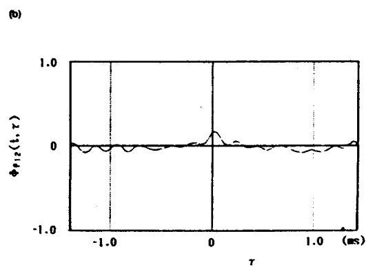
FIG.7 (a)Image-sources distribution, fall of sound field ( t :3-500ms). (b)Cross-correlation function [see Eqs.(8) and (9)], fall of sound field ( t :3-500ms).
