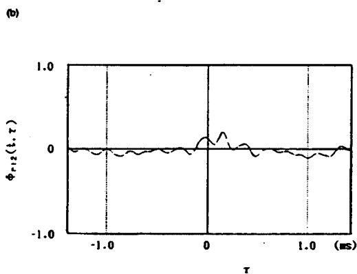
FIG.7 (a)Image-sources distribution, rise of sound field ( t :0-500ms). (b)Cross-correlation function [see Eqs.(8) and (9)], rise of sound field ( t :0-500ms).
