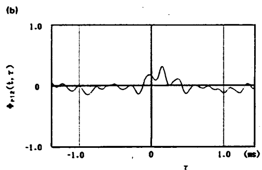
FIG.6. (a) Image-sources distribution, rise of sound field ( t : 0-100ms). (b) Cross-correlation function [see Eqs. (8) and (9)], rise of sound field ( t : 0-100ms).
